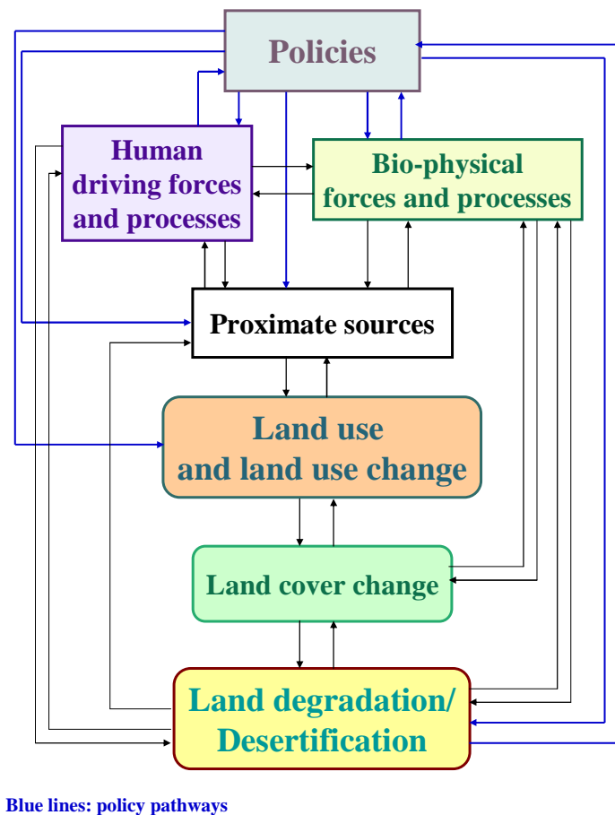
Figure 1. The land degradation/desertification sequence
